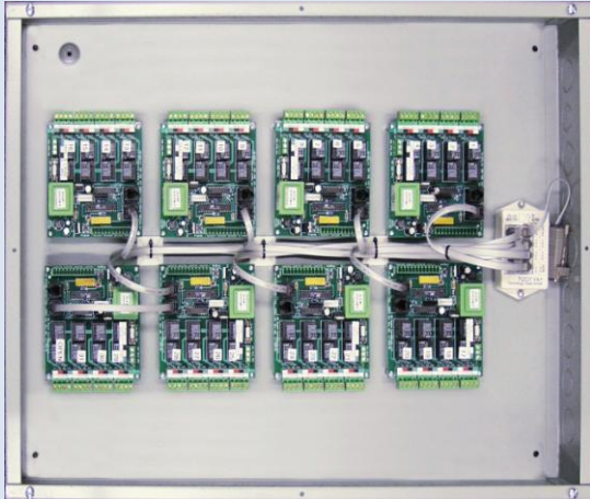
AC4 Installation (32 motors)
